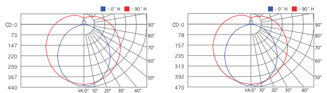
[ LTB16(built-in driver) / 5000K / 130° ]
